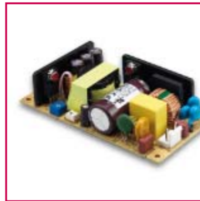
CPAmed60 S
