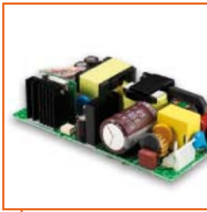
CPA100 S
